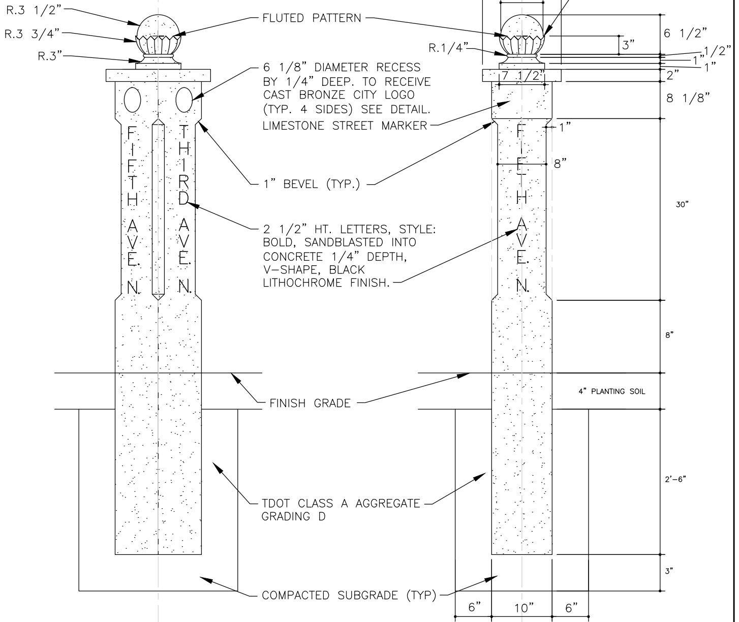
ELEVATION AT 45°
