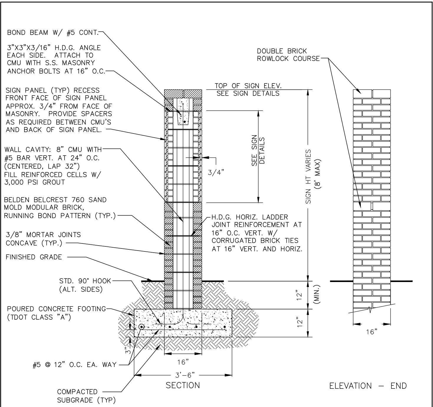
SECTION ELEVATION - END
